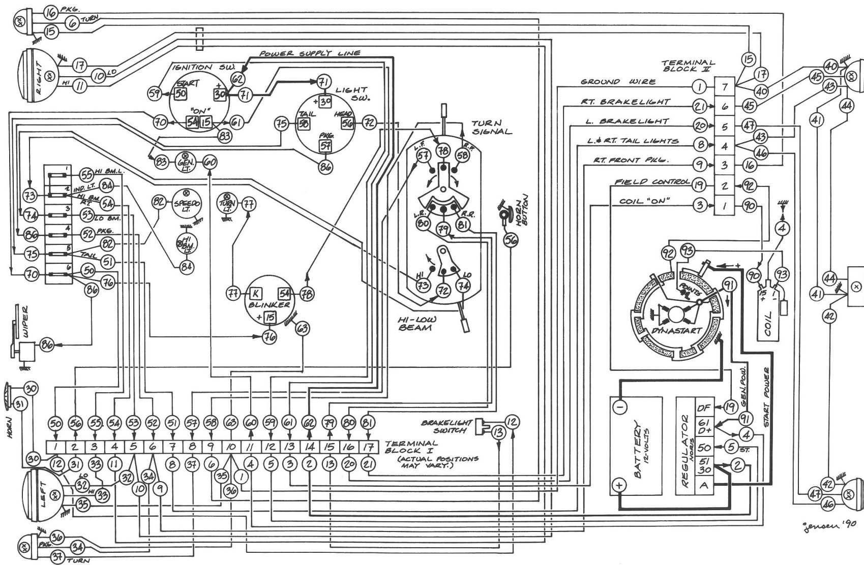
Electrical Schematic for US Export Isetta (circa 1958) from Isetta Restoration © John Jensen 1991
